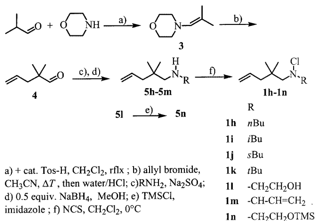
Scheme 2. Synthesis of chloroamines 1h–1n
