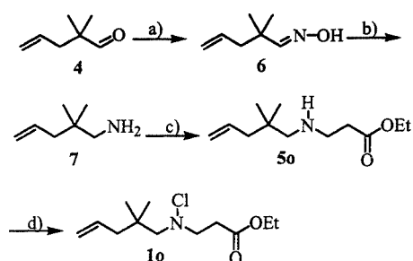
Scheme 3. Synthesis of chloroamine 1o
